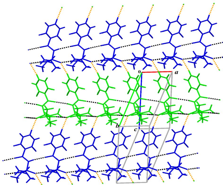
Fig. 3. Part of the crystal packing of studied structure is shown. A 2D layer is formed by connection of the independent chains (colored blue and green) through C–H...O=P hydrogen bonds (shown as orange dashed lines) parallel to the (04–4) plane.
