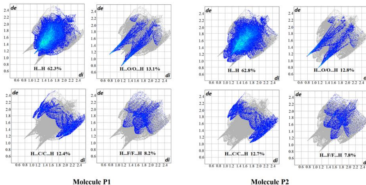
Fig. 5. Decomposed fingerprint plots and percentage contributions of various intermolecular H...H and H...X/X...H (X = O, C and F) contacts to the Hirshfeld surfaces of molecules P1 and P2. The full fingerprint plot appears as a grey shadow below each decomposed plot.
