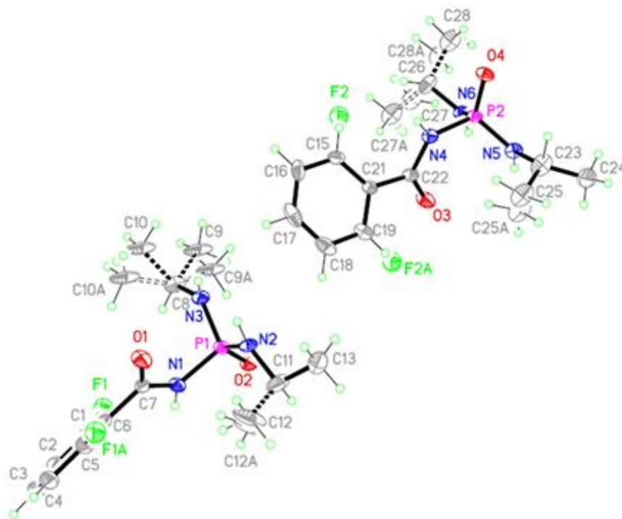
Fig. 1. The asymmetric unit of studied compound, showing the atom-labelling scheme for two molecules P1 and P2. Displacement ellipsoids are drawn at the 50% probability level and H atoms are drawn as circles of arbitrary radii. The minor disordered atoms with lower occupancy are labeled with the suffix 'A'.
