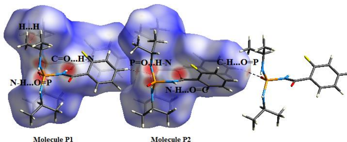
Fig. 4. A View of d_{\text{norm}} Hirshfeld surfaces plotted on the molecules P1 and P2 of the studied structure, surrounded by neighboring molecules associated with close contacts. The red spots are introduced by N-H...O, C-H...O and H...H interactions.
