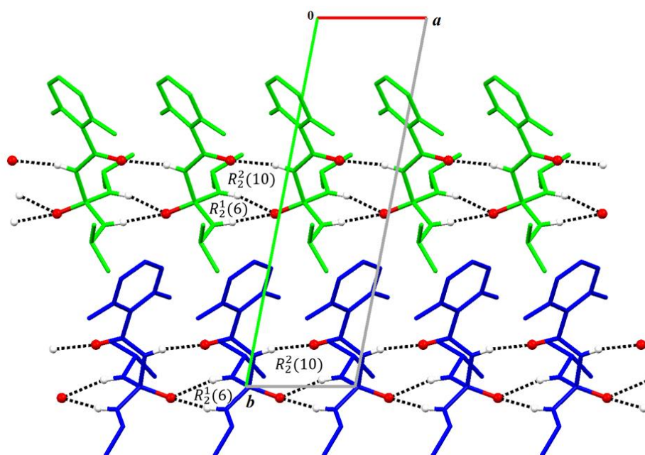
Fig. 2. A crystal packing diagram for studied structure is shown. 1D chains, along [100], are formed by the connection of adjacent independent molecules, via N CP –H \cdots O=C and [N–H] 2 \cdots O=P hydrogen bonds (black dashed lines) building R_2^2(10)/R_2^1(6) ring motifs. Different colors are shown for different molecules P1 and P2. The contact atoms O and H are displayed as “balls” style and H atoms not involved in hydrogen bonding have been omitted for clarity.
